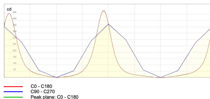
LINEAR INTENSITY DISTRIBUTION DIAGRAM
